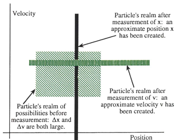
Fig. 9. The effect of a position measurement, or of a velocity measurement, is to create a position or velocity for the measured particle.
